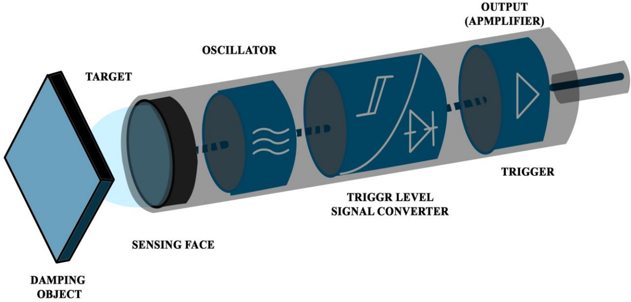
Fig.2 Internal elements of inductive proximity sensors
