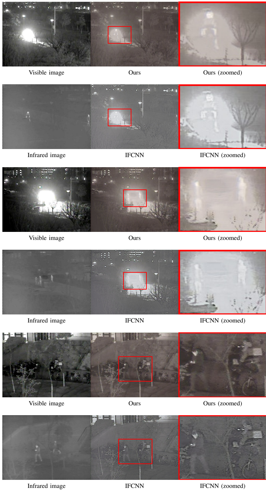
Figure 4: Qualitative results on the VIFB dataset.
