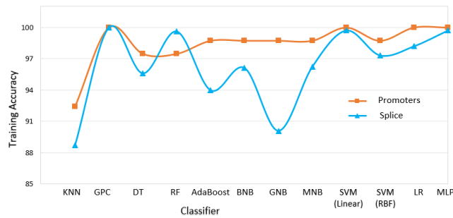
(a) Performance on training set
