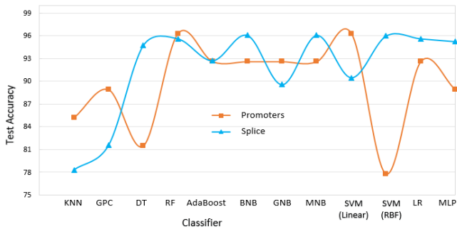
(b) Performance on test set
