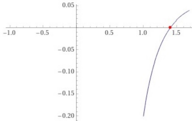
Fig. 2 Roots of H_4(x) [7]
