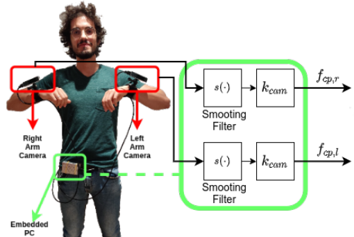
Fig. 3. The TPO suit , the motion tracking interface used to gather operator arm movements and generate virtual forces f_{cp}
