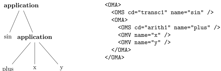
Figure 2: Syntax tree of the expression \sin(x + y) and its OpenMath-XML encoding
