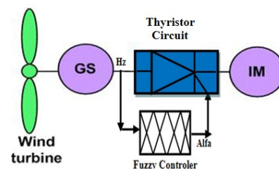
Fig. 1. System with voltage- frequency dependency fuzzy controller
