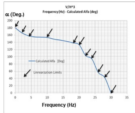
Fig. 6. Relations between firing angle “ \alpha ” and the “frequency based on V/Hz 3 Characteristic
