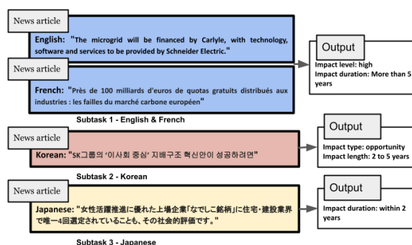
Figure 1: Overview of the ML-ESG3 task
