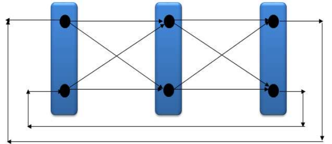
Fig. 1. Tail Biting Recurrent Layered Network
