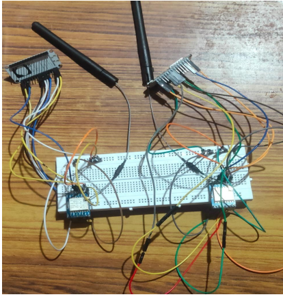
Figure .2. Module setup for small distance
