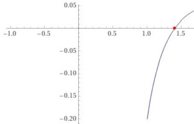
Fig. 2 Roots of H_4(x) [7]
