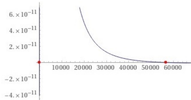
Fig. 1 Roots of H_2(x) [6]
