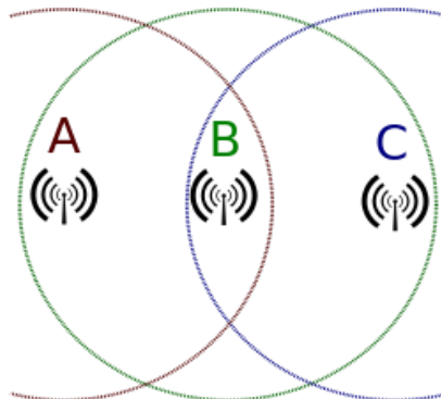
Fig. 3 Architecture for Hidden node problem
