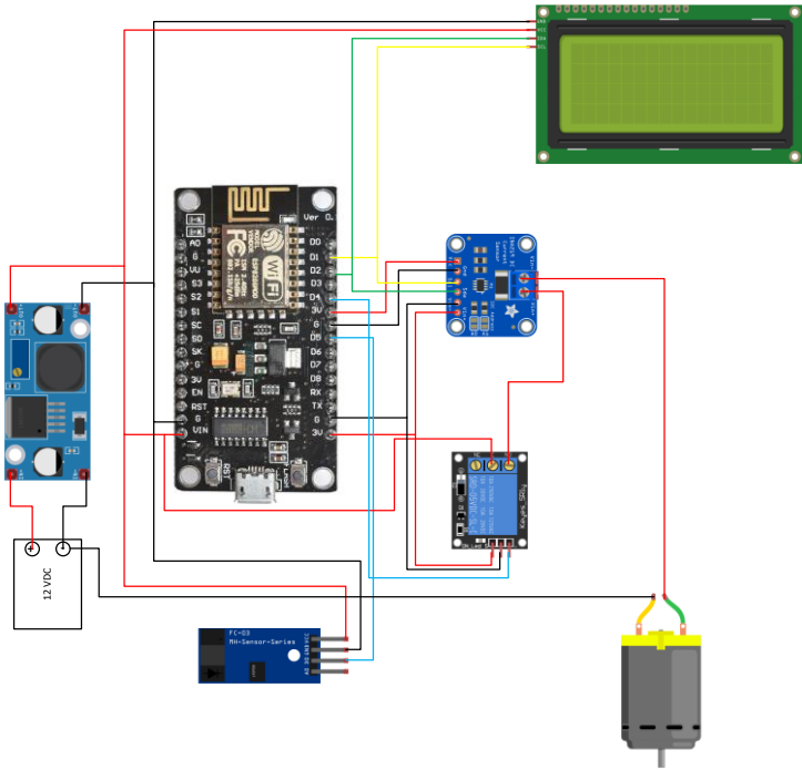
Figure 6. Wiring Diagram
