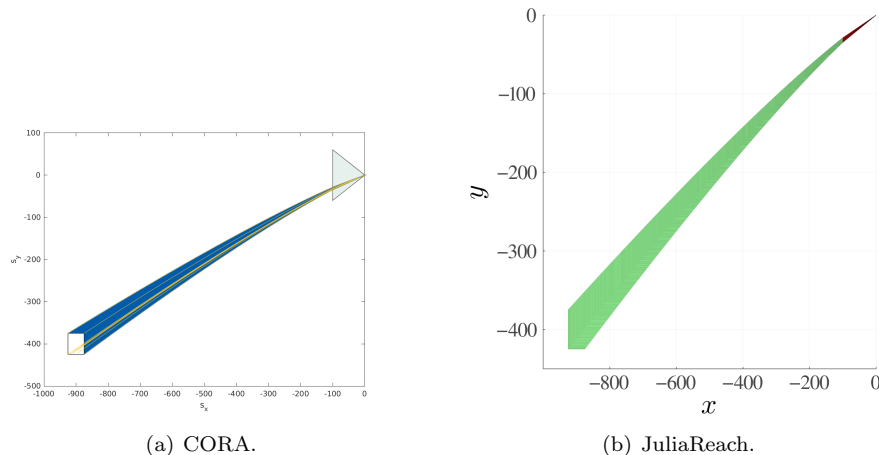
Figure 7: Reachable sets for the spacecraft rendezvous benchmark in the s_x - s_y -plane for the benchmark variant without maneuver abortion (SRNA01).
