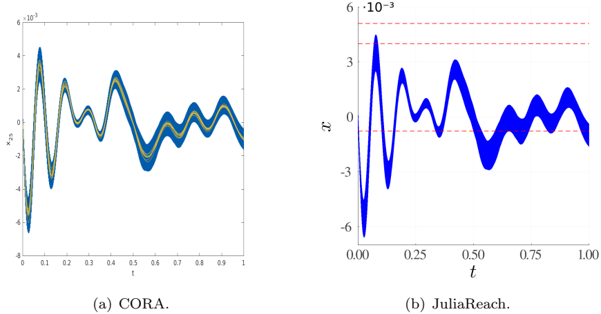
Figure 11: Building (BLDF01): Reachable sets of x_{25} plotted over time up to time 1. Some tools additionally show possible trajectories.
