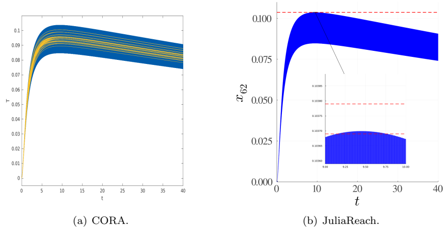
Figure 1: Heat3D: Reachable sets for the temperature at the center of the block over time for benchmark version HEAT01. Some tools additionally show possible trajectories.
