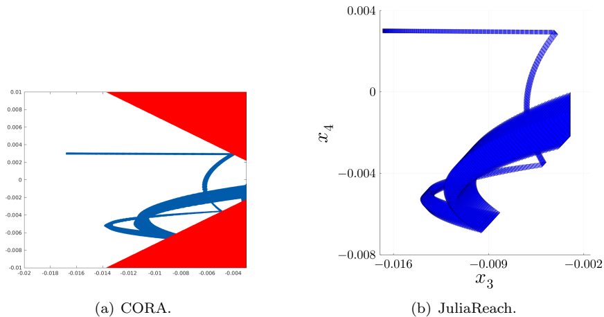
Figure 19: Gearbox (GRBX01): Reachable sets of x_3 and x_4 .
