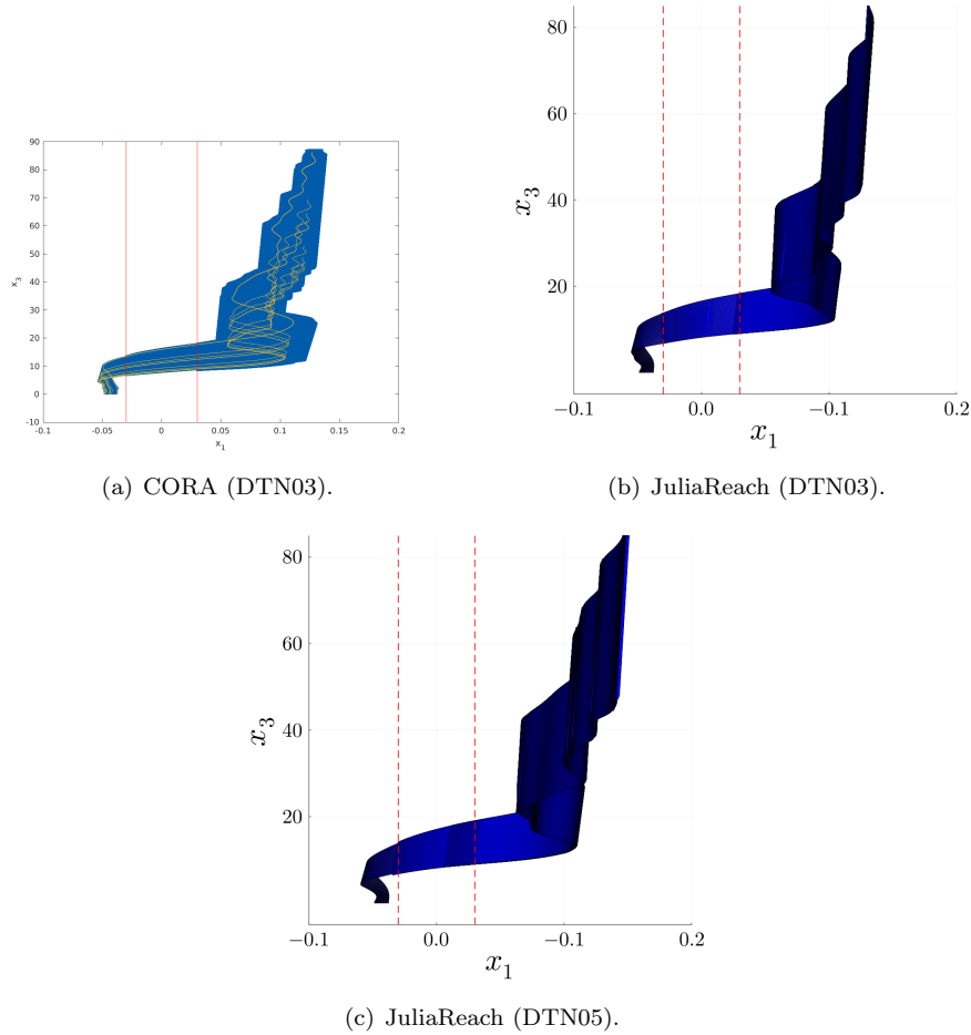
Figure 10: Reachable sets in the x_1 - x_3 -plane.
