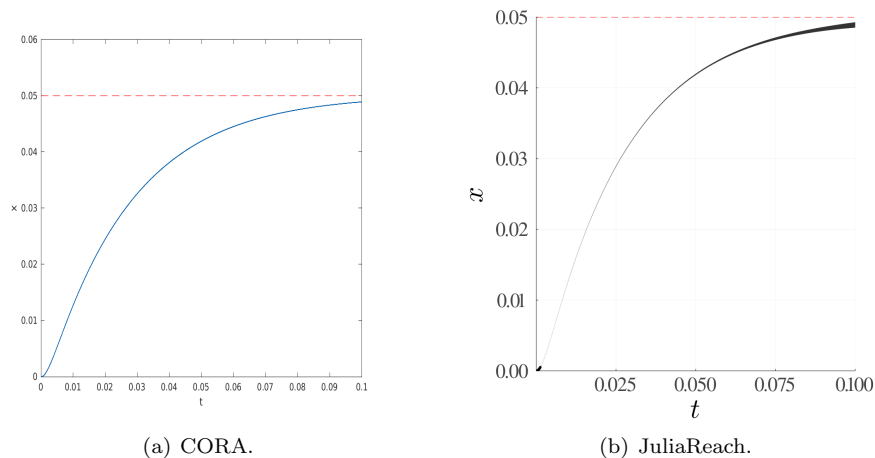
Figure 21: Brake: Reachable sets for x over time. Some tools additionally show possible trajectories.
