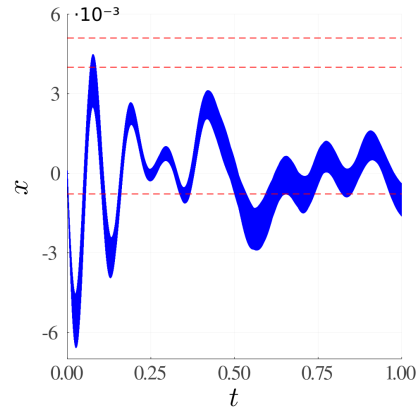
(b) JuliaReach.
