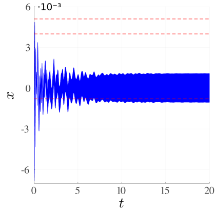
(b) JuliaReach.
