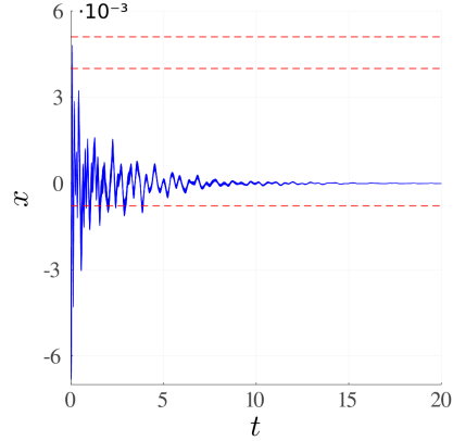
(b) JuliaReach.
