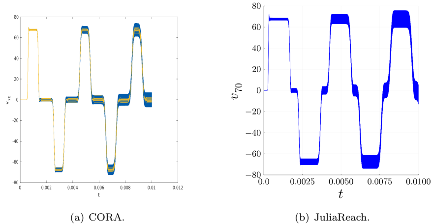
Figure 3: Clamped Beam CBF01: Reachable sets for the velocity at node 70. Some tools additionally show possible trajectories.
