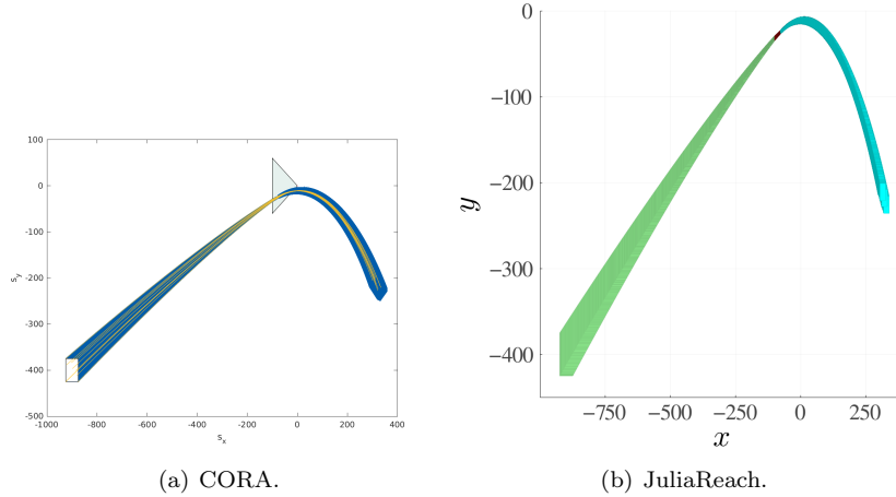
Figure 8: Reachable sets for the spacecraft rendezvous benchmark in the s_x - s_y -plane for the benchmark variant with maneuver abortion at t = 120 [min] (SRA01, over analysis time horizon of 300 [min])
