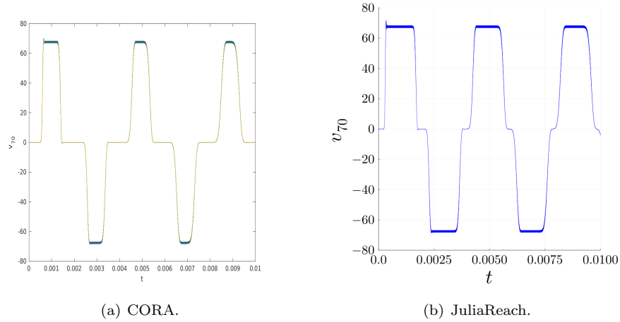
Figure 2: Clamped Beam CBC01: Reachable sets for the velocity at node 70. Some tools additionally show possible trajectories.
