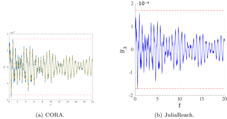
Figure 5: ISS: Reachable sets of y_3 plotted over time for the constant input case.
