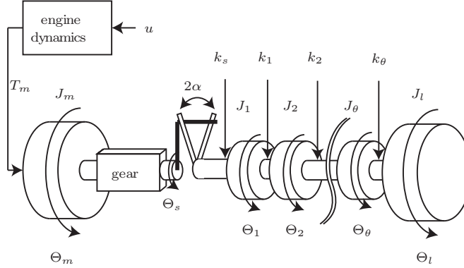
Figure 9: Powertrain model.
