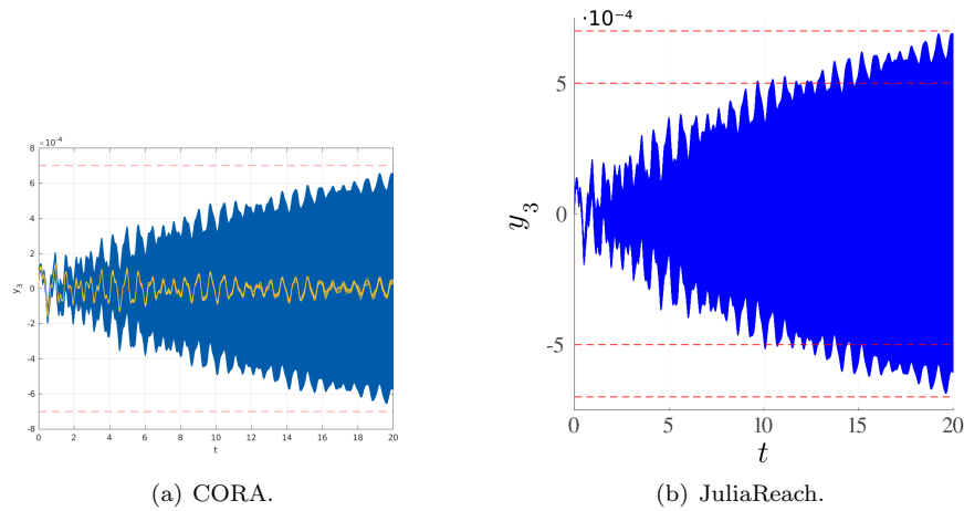
Figure 4: ISS: Reachable sets of y_3 plotted over time for the uncertain input case.
