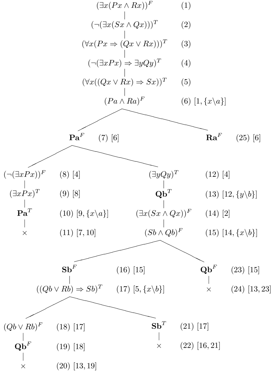
Figure 4: A derivation for SYN054+1 in the tableau calculus
